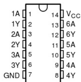
74HC04 & 74HC14 Six inverters
