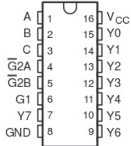
74HC138 3-to-8 Binary Decoder
