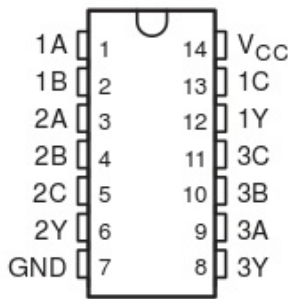
74HC10 Triple 3-input NAND
