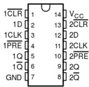
74HC74 Dual D-Flip/Flop
