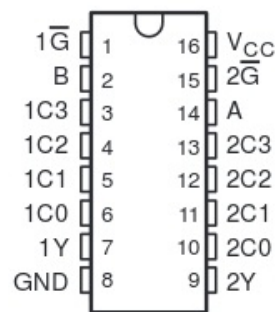
74HC153 Dual 4 -to-1 Multiplexer
