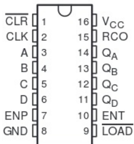
74HC163 4-bit Binary Counter
