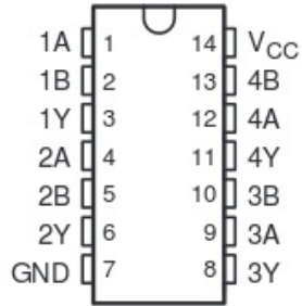
74HC00 Quad 2-input NAND
