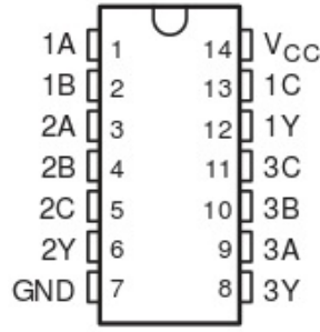
74HC27 Tripple 3-input NOR
