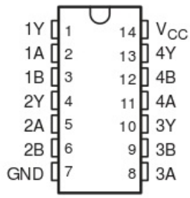
74HC02 Quad 2-input NOR
