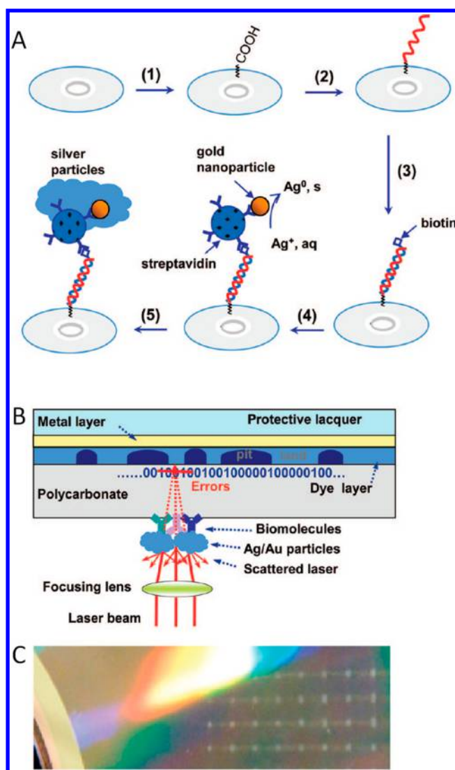
Figure 4. (A) Preparation of disc-based bioassay and signal amplification using gold/silver staining. (1) UV/ozone activation to generate carboxylic acid groups on CD surface; (2) immobilization of amino-tethered DNA probe strands via amide coupling; (3) hybridization with biotinylated DNA target strands; (4) binding of gold nanoparticle–streptavidin conjugates; (5) reductive precipitation of silver particles for signal enhancement. (B) Digital reading of bioassay using CD drive. The biomolecule/nanoparticle conjugates block the reading laser and generate errors. (C) Optical image of DNA microarray formed on a regular CD-R according to the above surface reaction and signal amplification. Reprinted with permission from ref 37. Copyright 2008 American Chemical Society.
